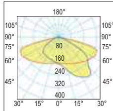
ST/CDL Stradale - Street optic LT-20320 5050
