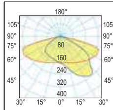
ST/CDL Optica stradale a richiesta On demand Street optic LT2032050508L
