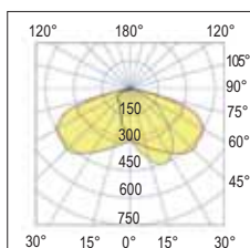
ST/CDL Stradale - Street optic
