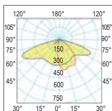
ST/CDL1 Optica stradale consigliata per strade con pista ciclabile Road optics recommended for roads with cycle tracks
