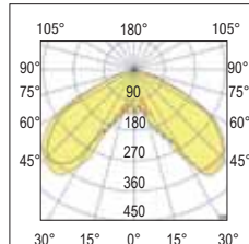
Optica STANDARD per illuminazione parchi - STANDARD optics recommended for lighting in parks LT-20485
