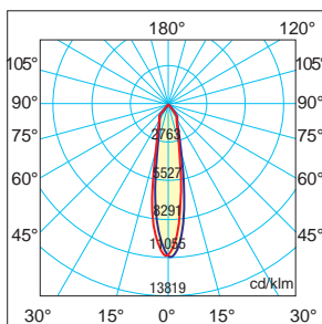
LED Retail - 25°
