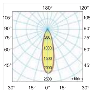
LED Retail - 40°
