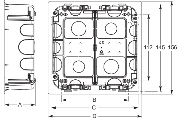
Vertical flush centralization boxes
