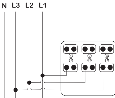
3 poles switch
